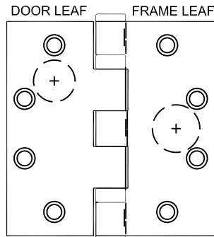
RIGHT HAND HINGE
