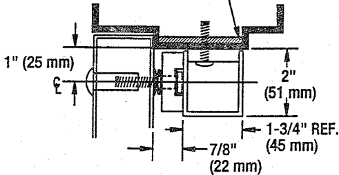
FIGURE 1A STANDARD INSTALLATION
